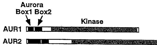
Fig. 1. Homology between human, Xenopus , Drosophila and yeast auroras. (A) The sequences for human aurora1 and aurora2 were deduced from full-length cDNA clones isolated from normal duodenum, pancreatic carcinoma and primary colorectal carcinoma libraries. Xenopus p46B (PIR:S53343), Drosophila aurora (PIR:A56220) and S.cerevisiae Ipl1 (SWISS-PROT:P38991) are included in the alignment. The alignment was generated by also including the two murine (DDBJ/EMBL/GenBank accession Nos D21099 and GB:U80932), an additional Xenopus (PIR:S53342) and two C.elegans (DDBJ/EMBL/GenBank accession Nos U53336 and U97196) sequences as input into msa, a parallel-coded multiple sequence alignment program that was run on MasPar MP2216 supercomputer. Boxed residues are common to three or more of the sequences; shaded residues represent regions of amino acid similarity between two or more sequences; overlines correspond to the conserved Aurora Box1 and Aurora Box2 sequences; the arrow denotes the start of the C-terminal serine/threonine kinase domain; the circled residue indicates the location of a single nucleotide polymorphism described in the text; solid circles correspond to the location of various yeast and Drosophila mutants (Francisco et al. , 1994; Glover et al. , 1995); and stars denote the site of the kinase-inactivating and -activating point mutants described in the text. (B) Schematic domain structure of human aurora1 and aurora2.
